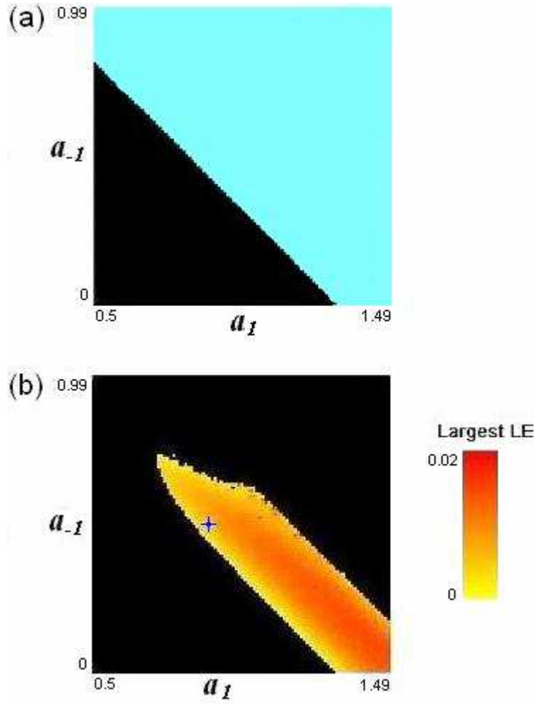
Figure 9. a) The region of parameter space for Eq. (2) where the Lyapunov function exists is shown in black (and the orbit must attract to an equilibrium point) and the region where complex dynamics is possible in blue. b) Black areas are where the orbit attracts to the equilibrium point. The black region in (a) closely matches the black region in the lower left of (b). In these scans a_2 = 0.451 and a_2 = 0.237 . The blue cross in (b) shows condition (3), considered throughout the paper.
