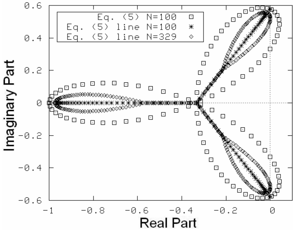
Figure 10. The eigenvalues for Eq. (5) exhibit a trefoil shape but those of the line system form a rotated Y at s = 1 and N = 100 . As the number of species in the lines increases, the eigenvalues seem to approach those of the ring. This may be due to the fact that an infinitely long line is indistinguishable from a ring to those species far from the ends.
