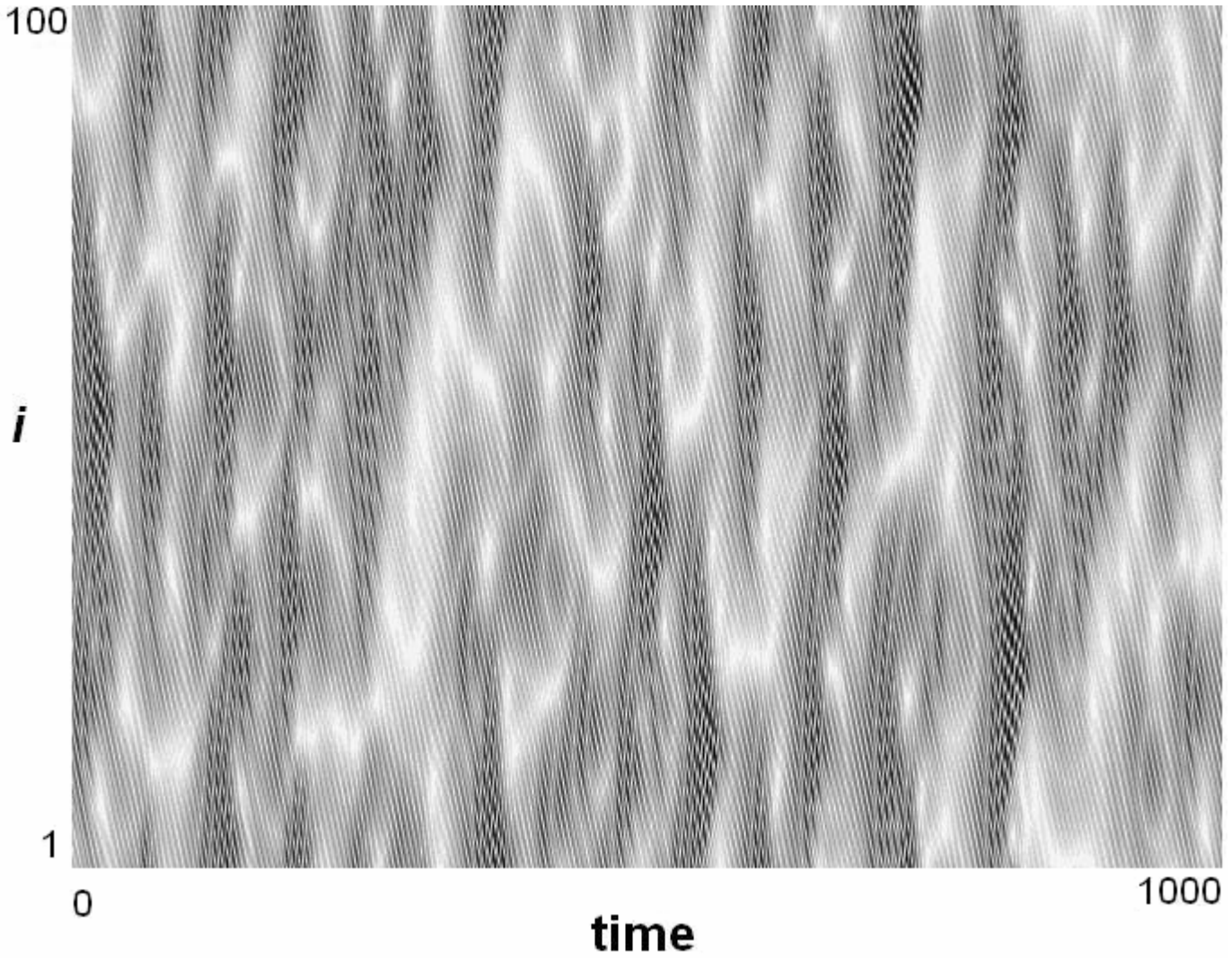
Figure 5. The magnitude of the spatial derivative |x_i - x_{i-1}| about the ring over time for Eq. (2) with N = 100 . The spatiotemporal chaos ensures that the patterns seen in the plot will never repeat. Although the equations describing the system are homogenous, the solution is heterogeneous and is an example of spontaneous symmetry breaking.
