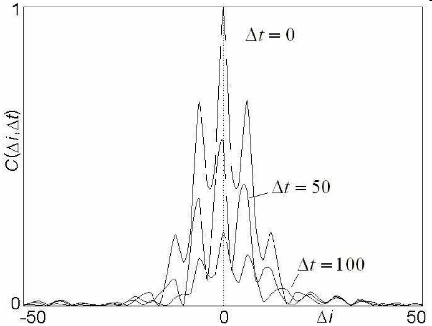
Figure 6. The spatiotemporal cross-correlation function plotted over i shows the propagation and dispersion common to Lotka-Volterra ring systems. The plot is not symmetric due to the asymmetry in the rows of the interaction matrix, though there does seem to be a spatial periodicity of \Delta i = 6 in both directions.
