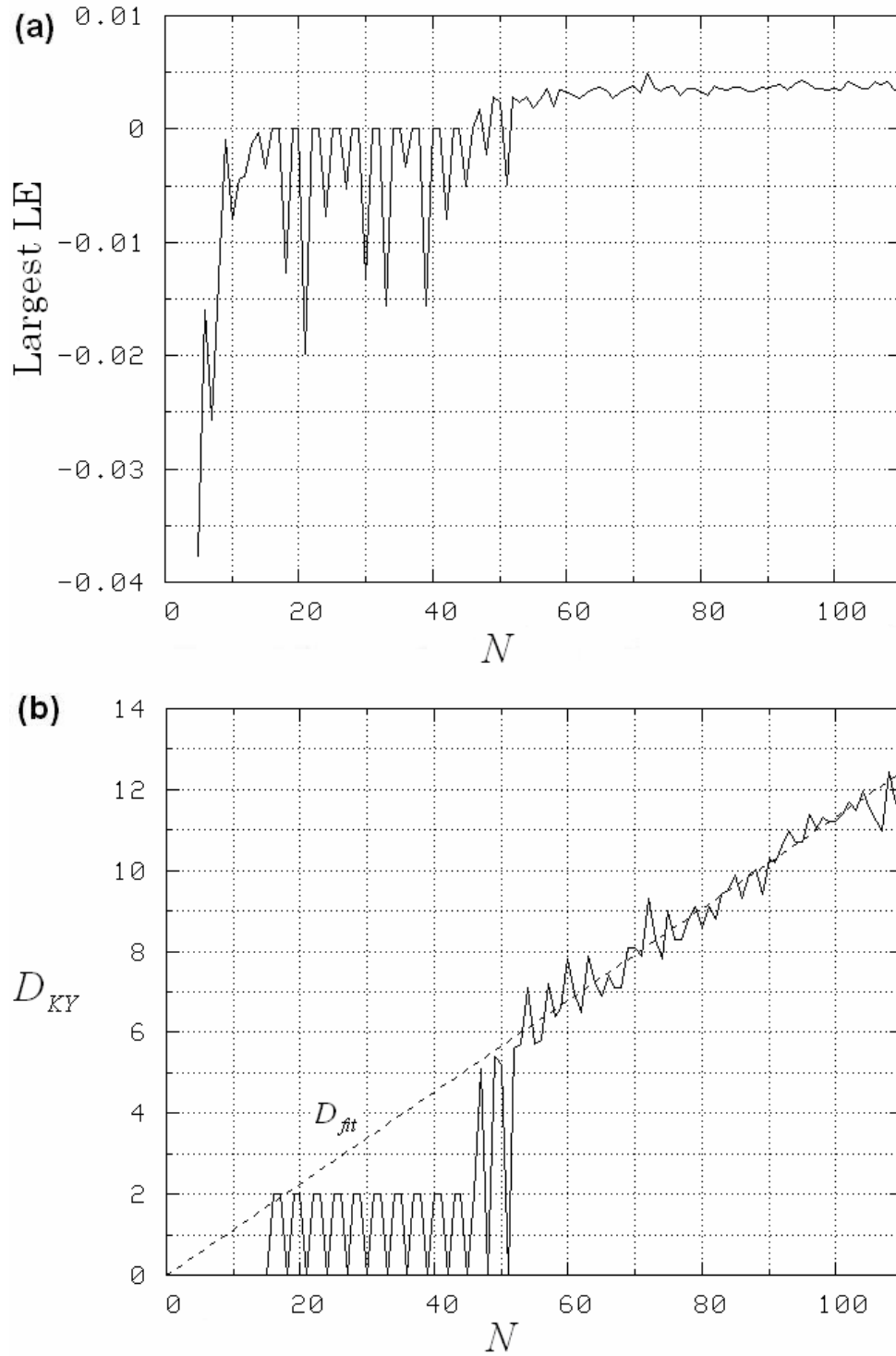
Figure 4. The dimensionality of the system N provides a discrete bifurcation parameter. a) The largest Lyapunov exponent oscillates between negative values and zero at low N and remains positive for N \geq 52 . b) The dimension of the attractor follows the largest Lyapunov exponent, oscillating between an equilibrium point and a 2-torus for small N , and is not an integer when the system is chaotic, indicating a strange attractor. A regression line fitted to the chaotic cases follows the equation D_{fit} = 0.11N - 0.01 .
