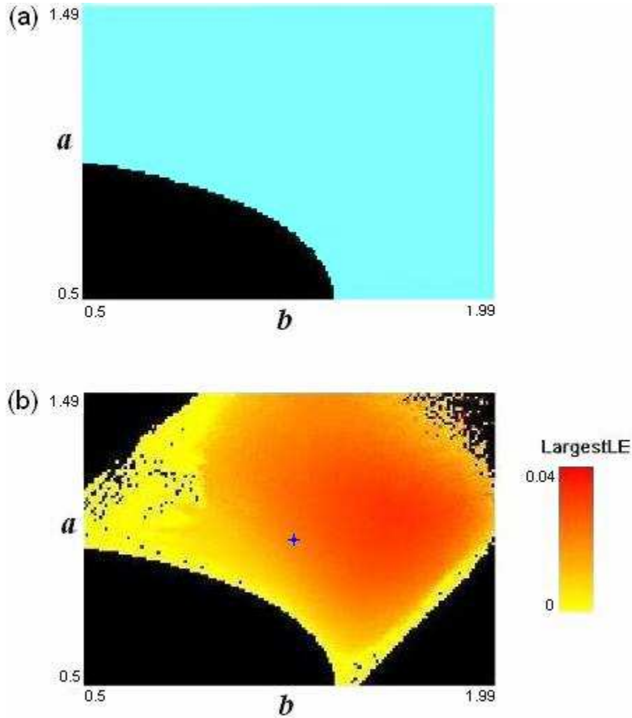
Figure 8. a) The regions of parameter space for Eq. (5) (with N = 100 ) where a Lyapunov function exists and therefore the orbit must approach an equilibrium point (black) and the regions where more complex dynamics are allowed (blue). b) The largest Lyapunov exponent over the same region of parameter space. The black regions represent parameter values where the orbit attracts to an equilibrium point (largest Lyapunov exponent less than zero). Notice how the region where complex dynamics is forbidden by the existence of a Lyapunov function in (a) closely matches the region where the orbit attracts to an equilibrium point in the lower left of (b). The blue cross in (b) shows a = b = 1 .
